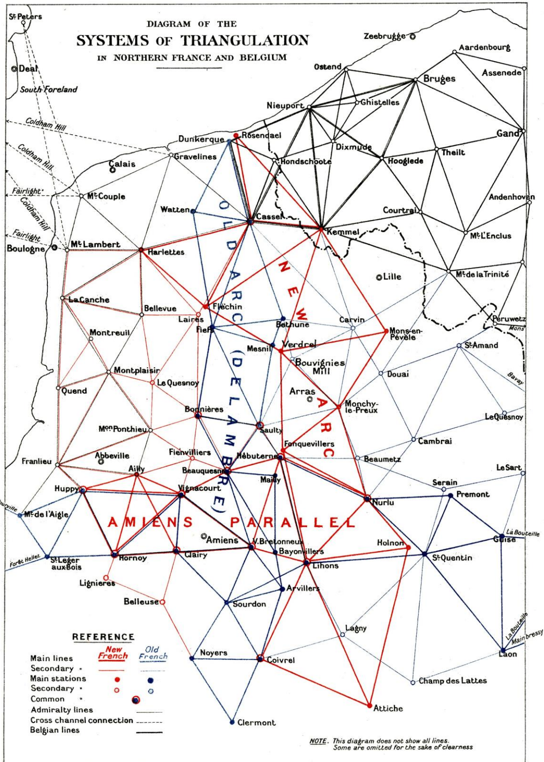
Diagram 1 Systems of triangulation in Northern France and Belgium.
