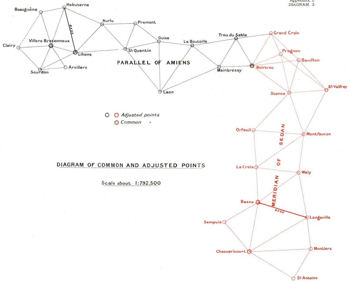
Diagram 3 Common and adjusted points.
