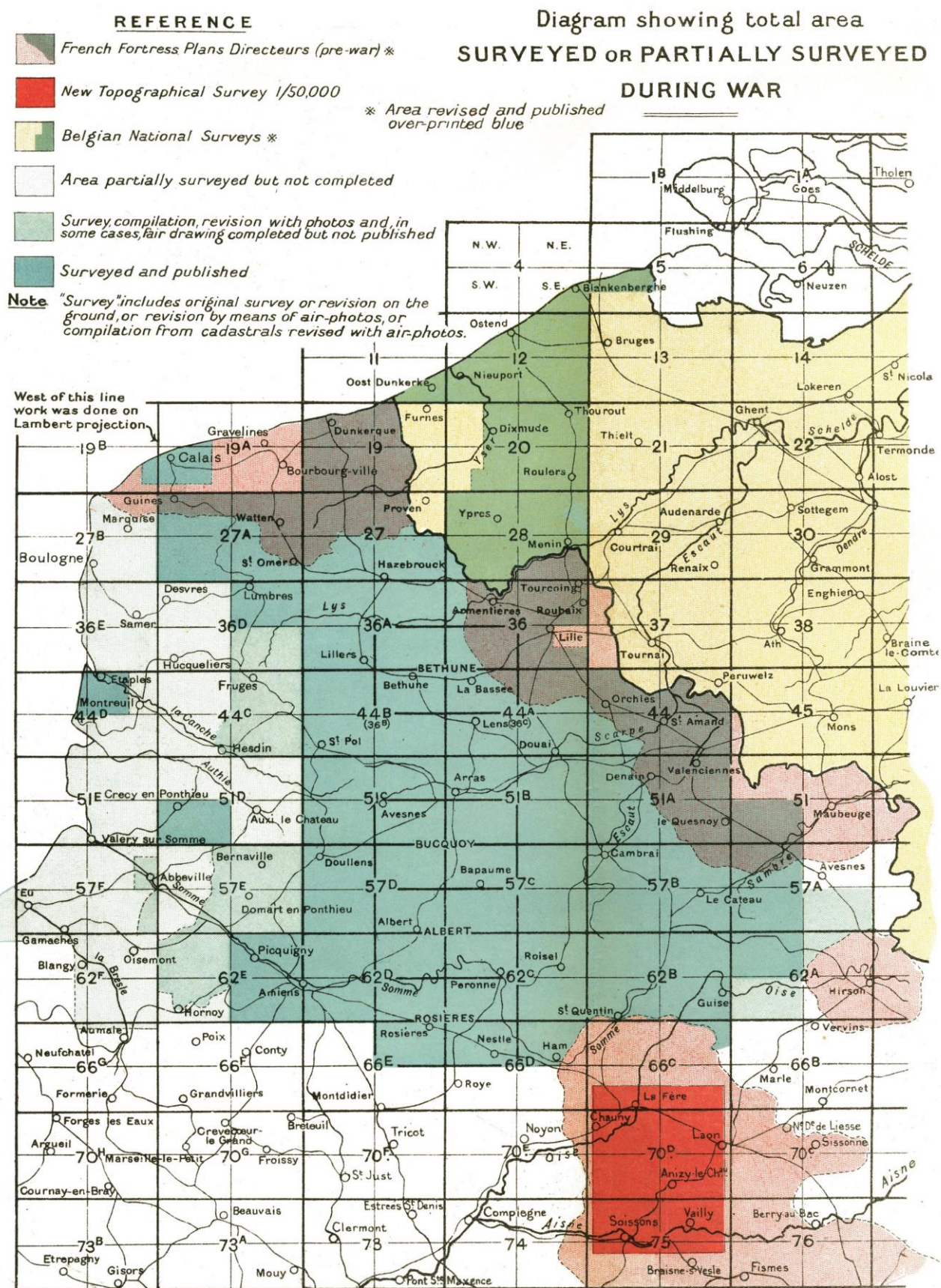
Diagram of area surveyed or partially surveyed during the war.
