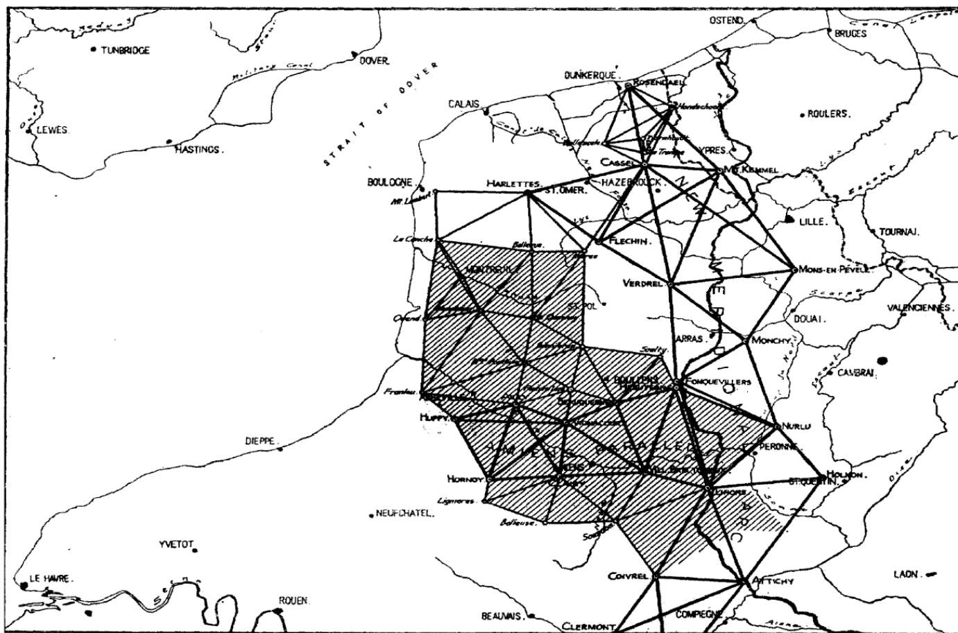
New British Surveys and connection between French and Belgian Triangulations
