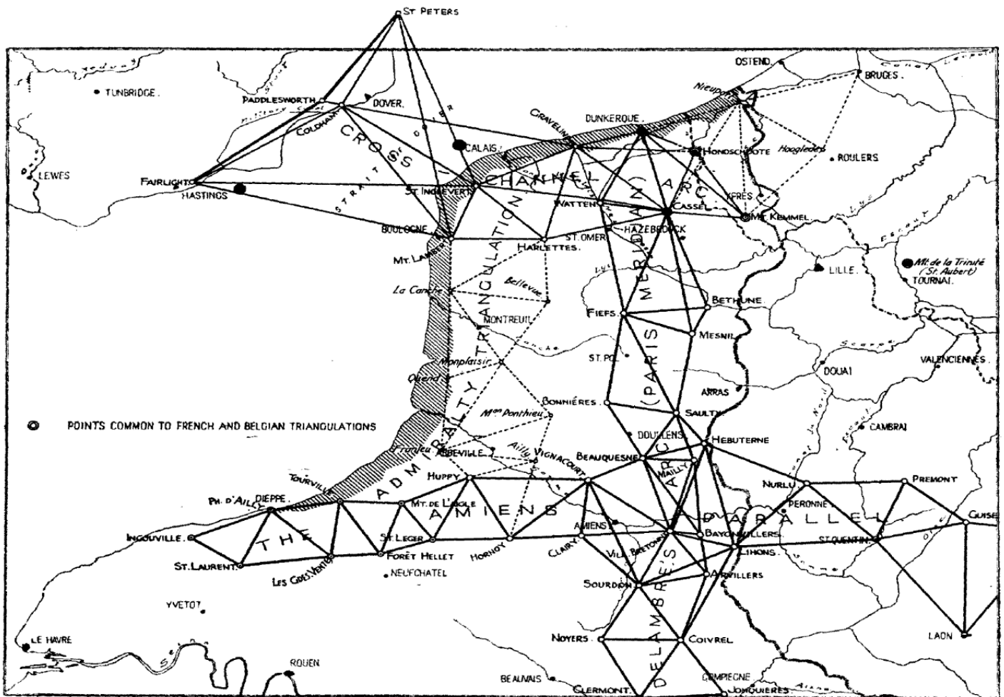
The French Geodetic Triangulation
